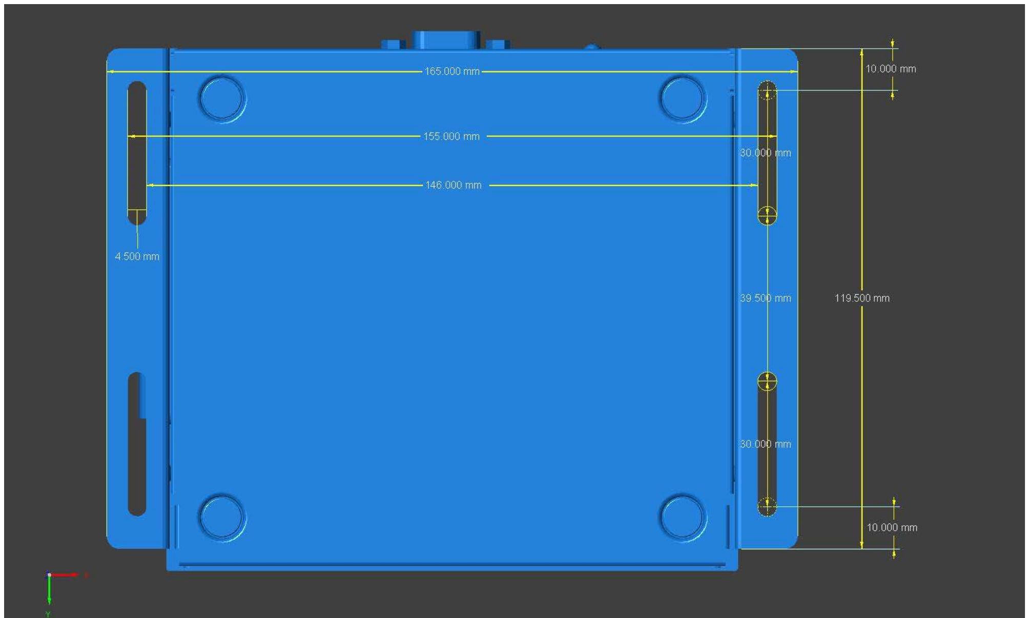
HD Series 2 Dimensions
